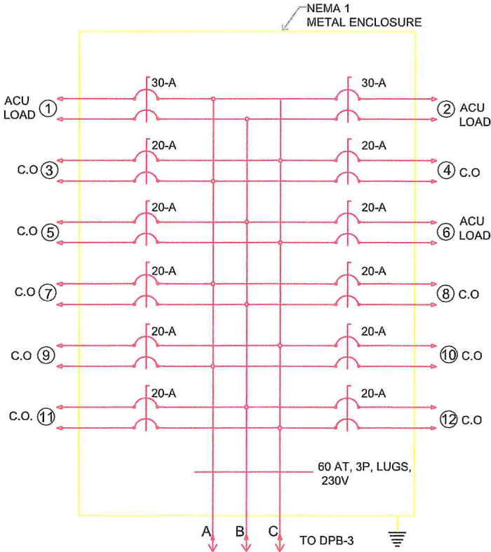
PP - 3 PANEL BOARD DETAILS
