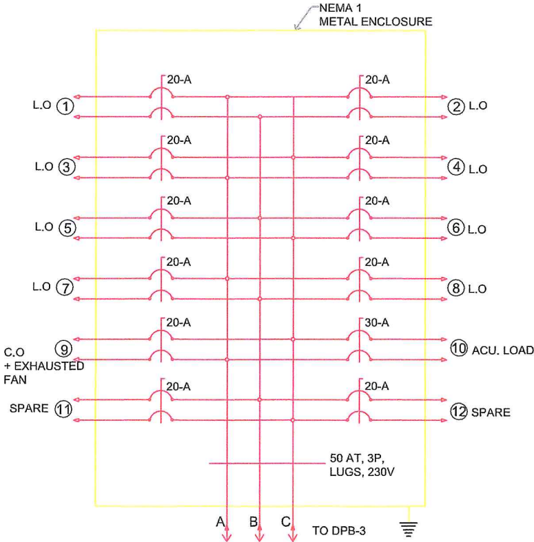
LP - 3 PANEL BOARD DETAILS
